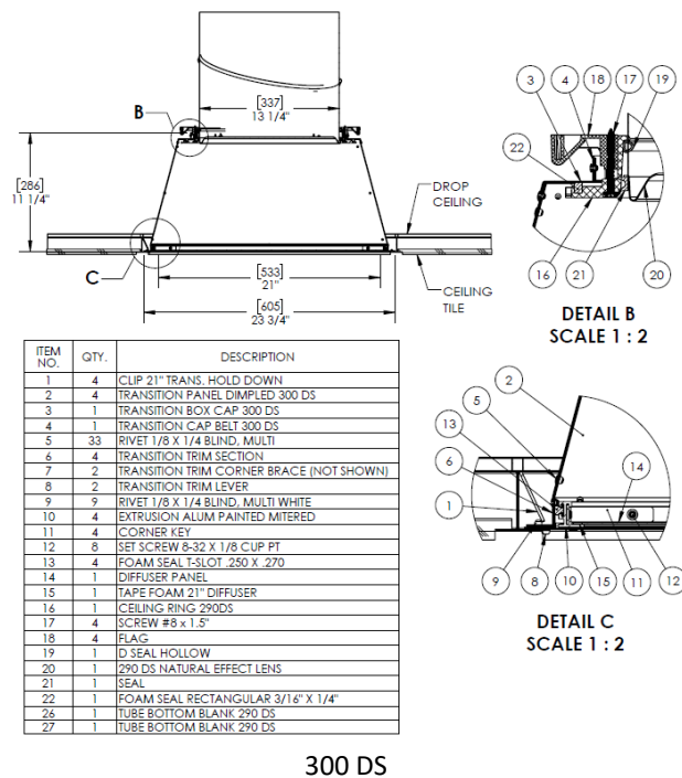
FIGURE 7 - TYPICAL SOLATUBE SQUARE TRANSITION ASSEMBLY FOR 300 DS, 330 DS, AND 750 DS
