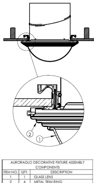
FIGURE 10 - SOLATUBE 160 DS AND 290 DS DECORATIVE FIXTURES
