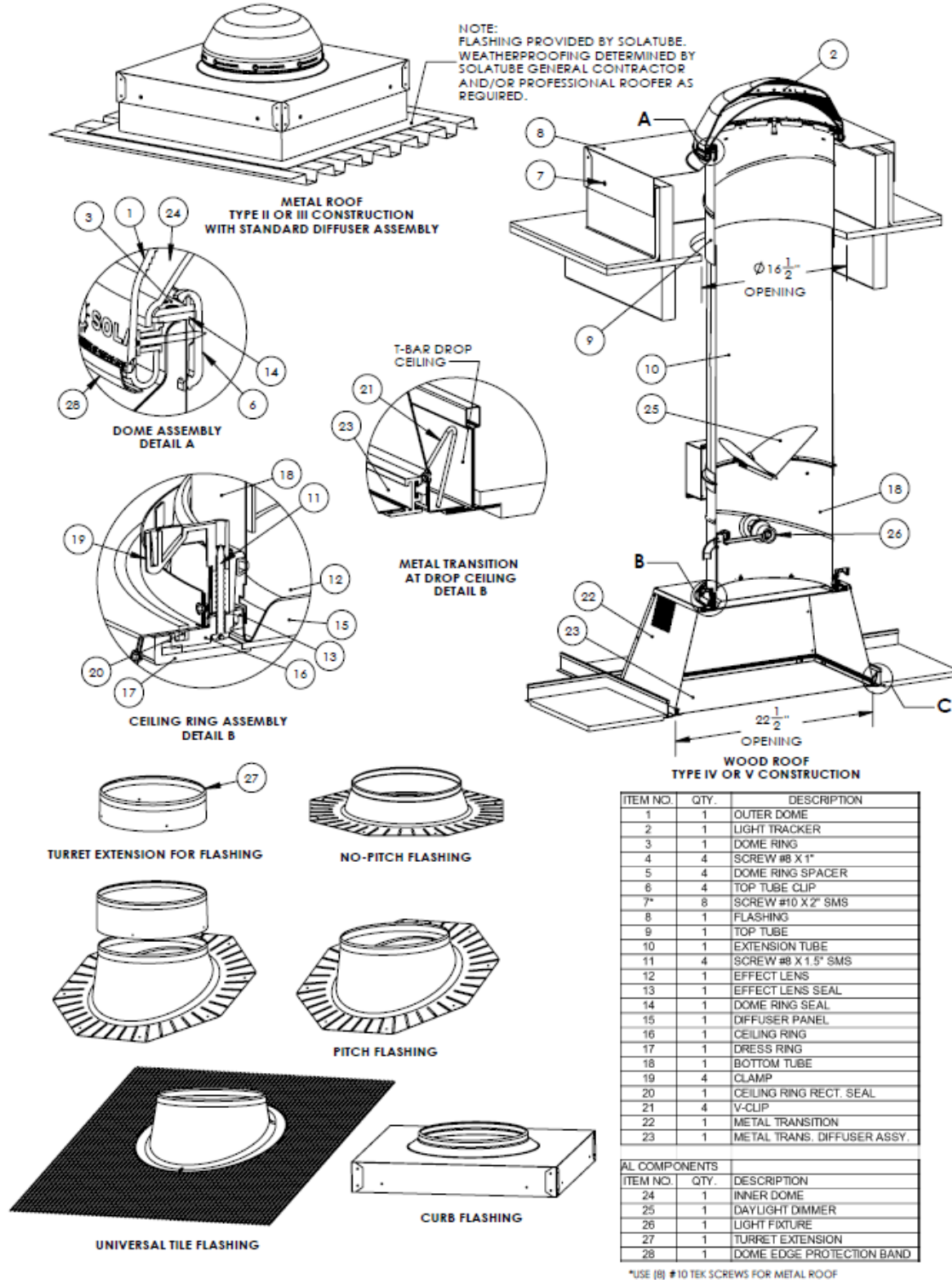
FIGURE 2 - 300 DS SOLATUBE WITH DETAILS
