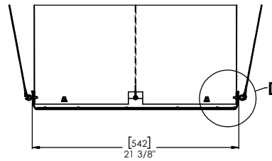
45° ROTATION ABOUT CENTER SECTION VIEW
