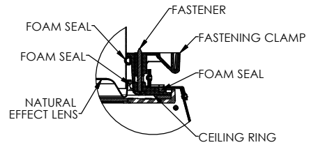
DETAIL D SCALE 3 : 1
