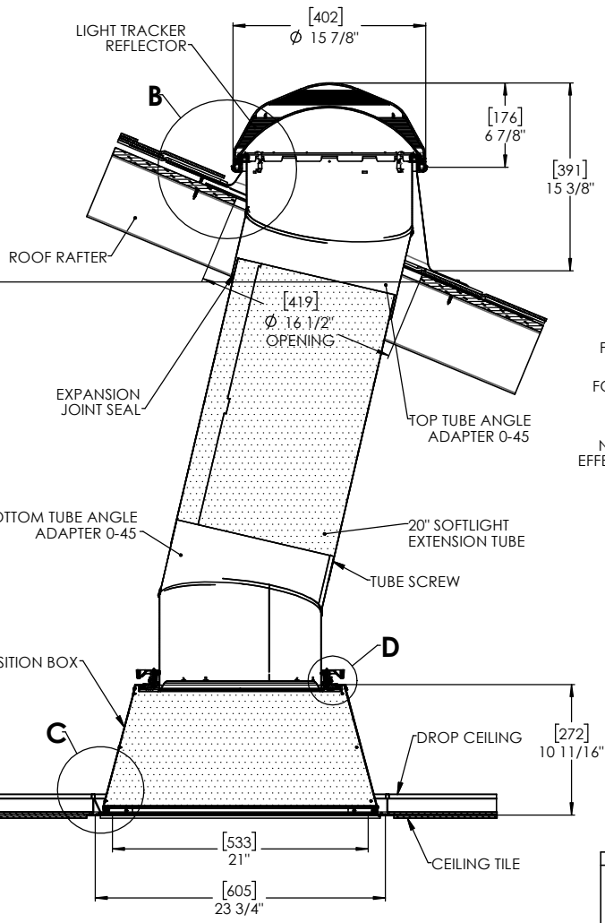
FULL SECTION SCALE 1:1
