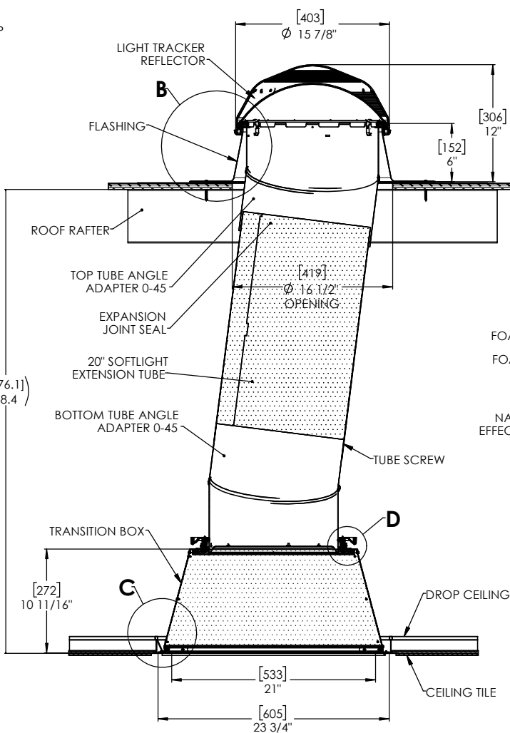
FULL SECTION SCALE 1:1
