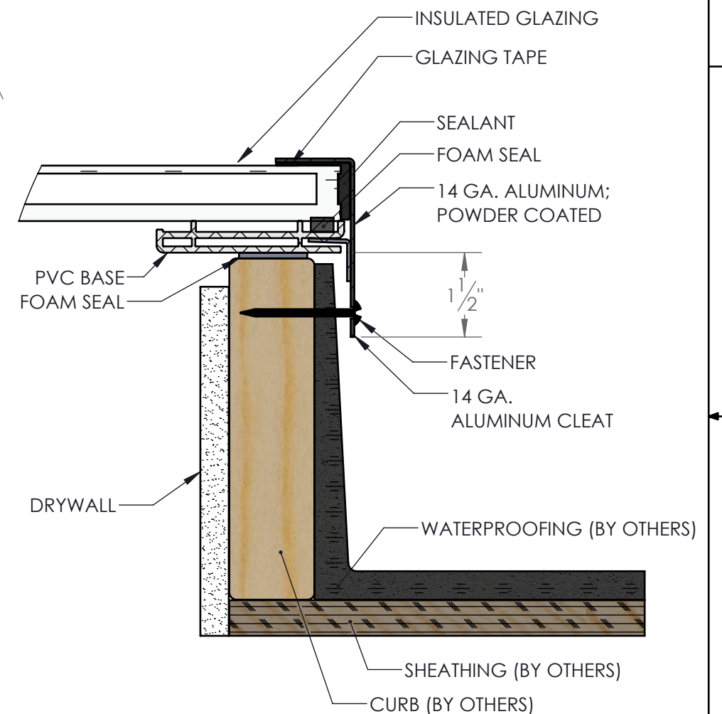
DETAIL A
