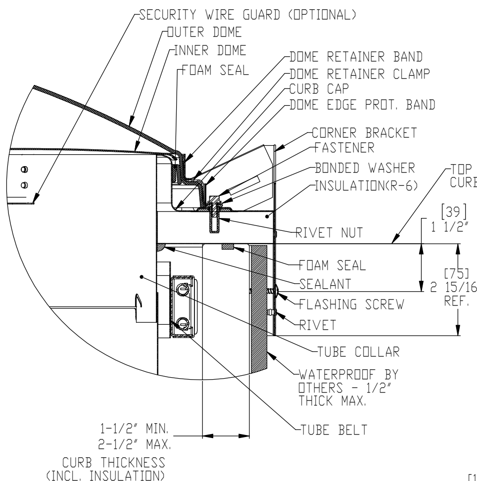
DETAIL B SCALE 3 : 1
