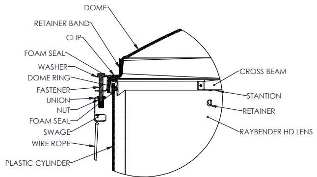
DETAIL C SCALE 3 : 1
