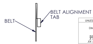
DETAIL H SCALE 8 : 1
