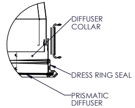
DETAIL E SCALE 2 : 1
