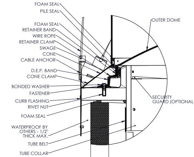
DETAIL C SCALE 3 : 1
