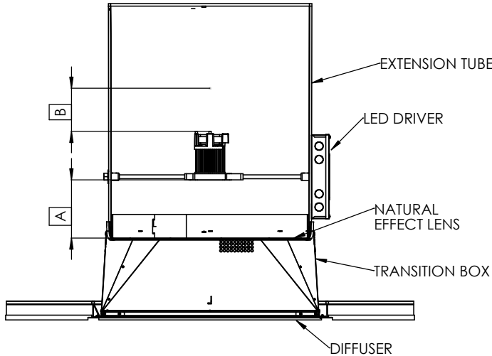
FULL SECTION SCALE 1:1
